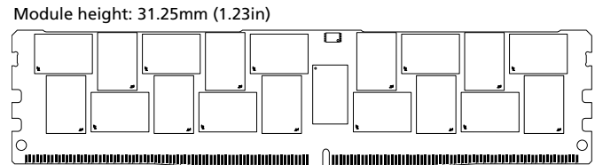
Figure 1: 288-Pin LRDIMM (MO-309, R/C-B, R/C-B1)
