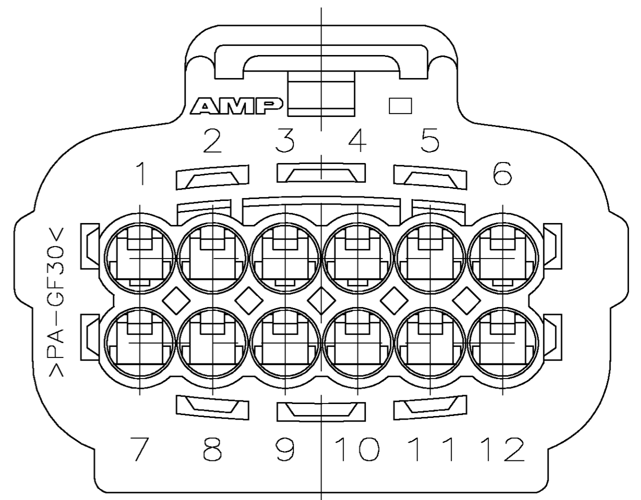
VIEW B-B
