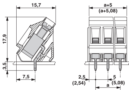
Dimensioned drawing
