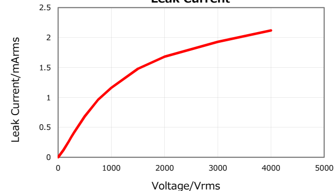
Leak Current
