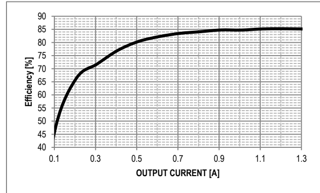
Figure 3. Efficiency vs. Output Load: V_{OUT\_RX} = 9V
