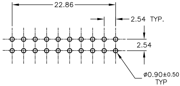
RECOMMENDED P.C.B. LAYOU
