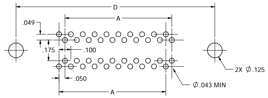
RECOMMENDED PCB LAYOUT COMPONENT SIDE
