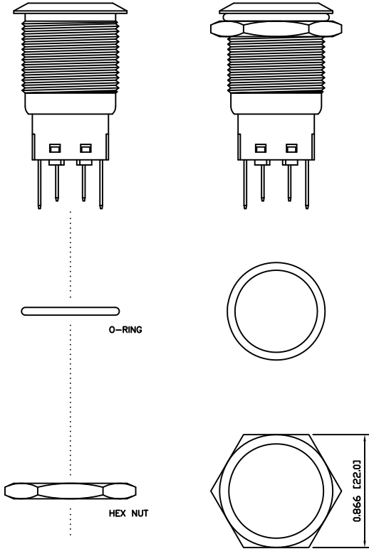
EXPLODED VIEW
