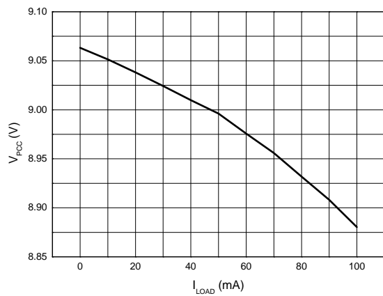
V PCC Load Regulation
