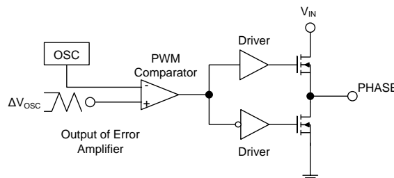
Figure 8.The PWM Modulator
