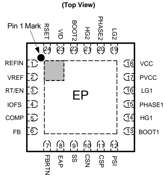
U-QFN4040-24 (FN Package)
