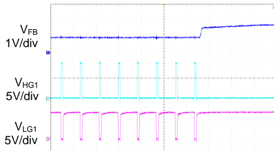
Time 4μs/div
