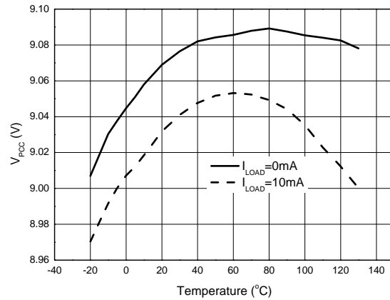
V PCC vs. Temperature
