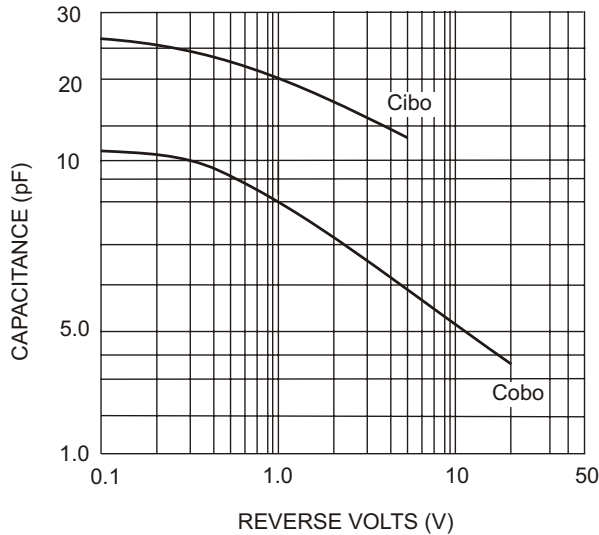
REVERSE VOLTS (V) Fig. 3 Typical Capacitance
