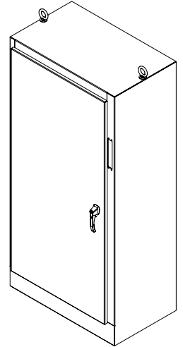
ISOMETRIC VIEW
