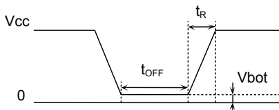
Figure 55. Rise waveform
