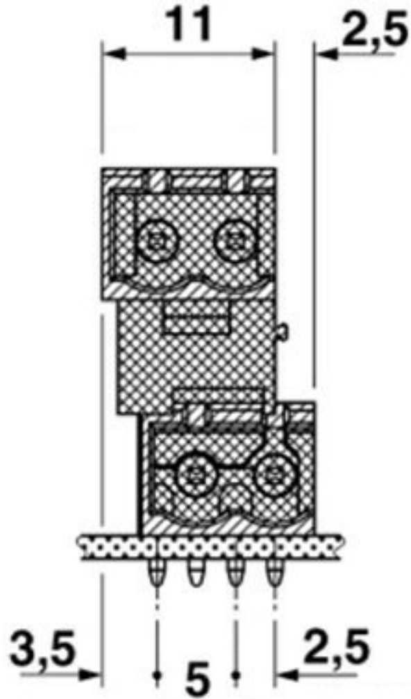
Dimensioned drawing
