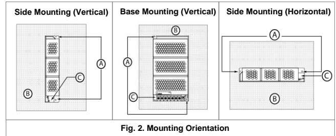
Fig. 2. Mounting Orientation
