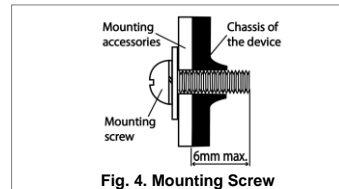
Fig. 4. Mounting Screw
