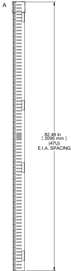
FRONT VIEW
