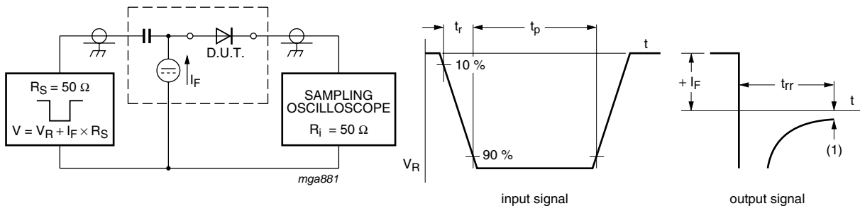
(1) I_R = 1\text{ mA} Input signal: reverse pulse rise time t_r = 0.6\text{ ns} ; reverse voltage pulse duration t_p = 100\text{ ns} ; duty cycle \delta = 0.05 Oscilloscope: rise time t_r = 0.35\text{ ns}
