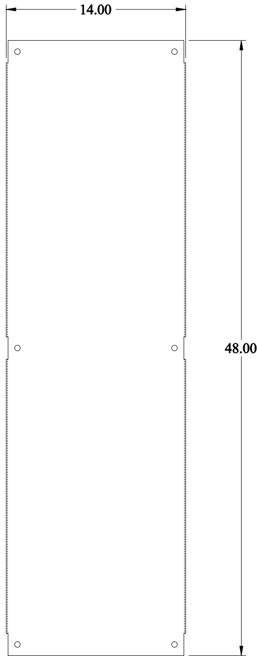
FRONT VIEW
