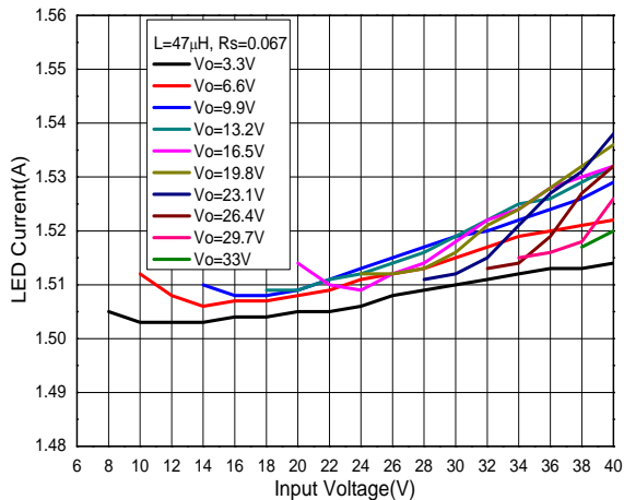
LED Current vs. Input Voltage (MSOP-8EP, R s =0.067Ω, L=47μH)
