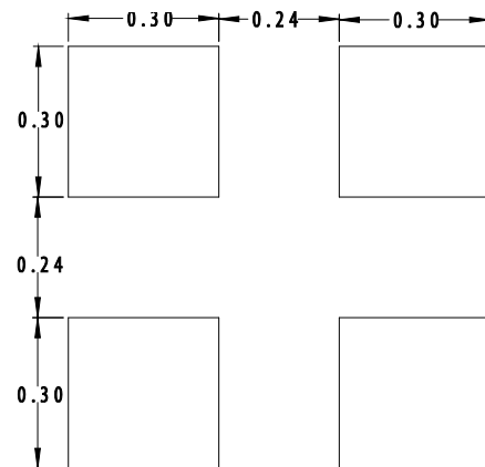
Figure 7: Recommended Soldering Land Pattern
