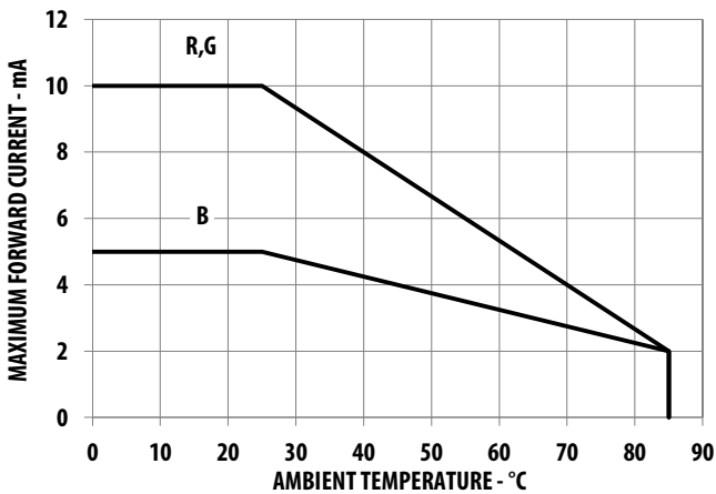
Figure 6: Derating Curve
