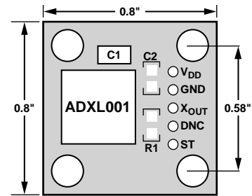
Figure 2. EVAL-ADXL001 Board Layout
