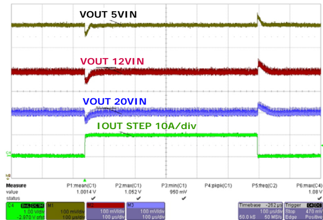
FIGURE 15. LOAD TRANSIENT (0A TO 10A STEP, SLEW RATE = 10A/μs) FOR INPUT = 5, 12, 20V
