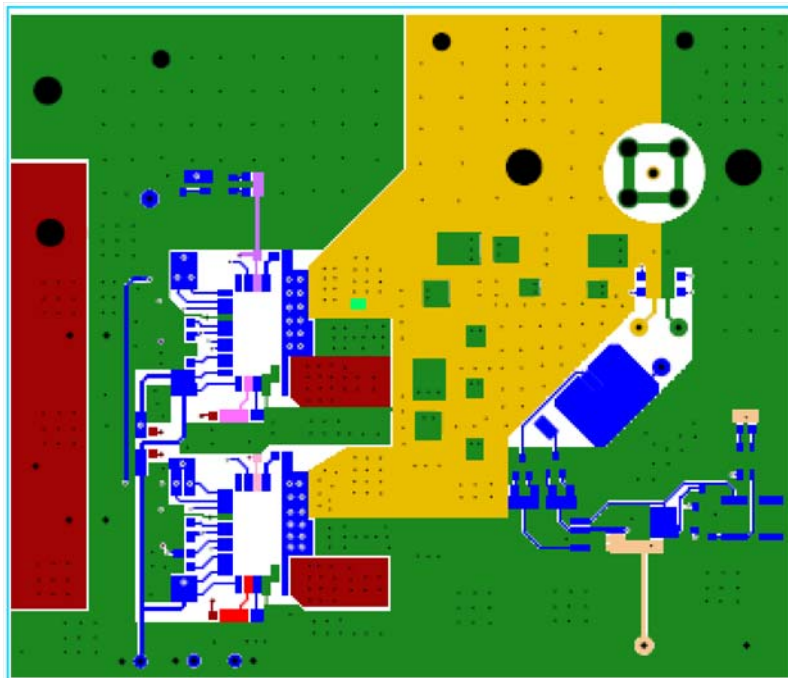
FIGURE 5. TOP LAYER
