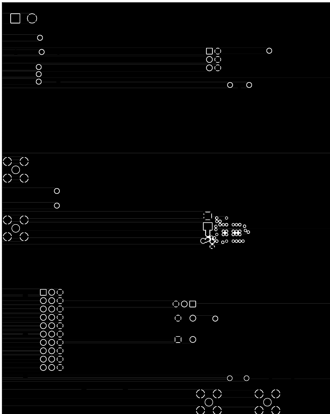
Figure 10. Si5318-EVB—Layer 8, Bottom
