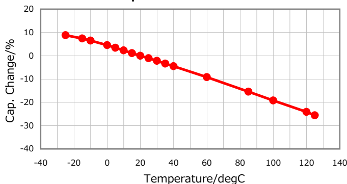
Temperature Characteristic
