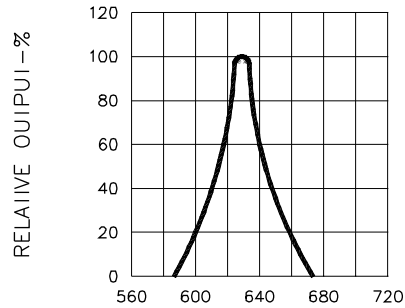
WAVELENGTH ( \lambda ) - nm Fig.2 SPECTRAL RESPONSE
