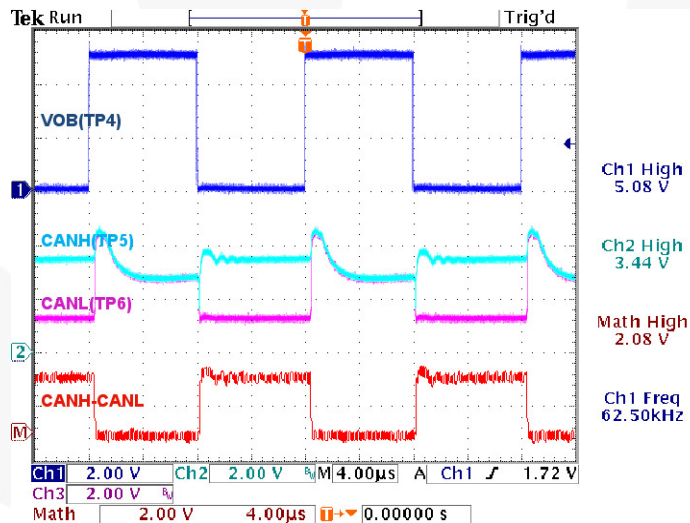
Figure 5. DRIVER_EN and VINB are Input Signals; FOD8012 Output Signal, VOB, Drives RS485 Transceiver
