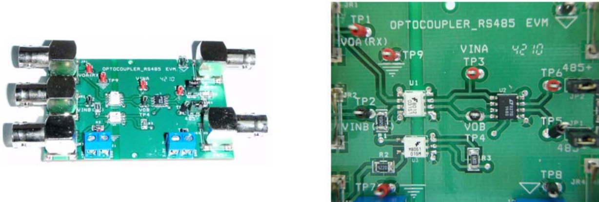
Figure 2. Photographs of the FEBFOD8012_RS485 Board
