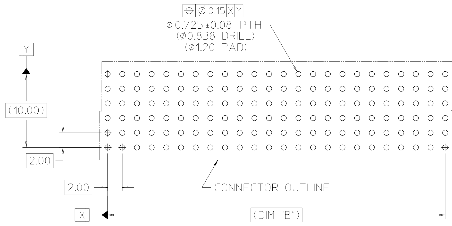
PCB LAYOUT: COMPONENT SIDE
