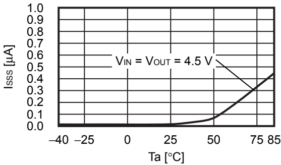
(5) Current consumption during power-off ( I_{SS3} ) vs. Temperature ( T_a )
