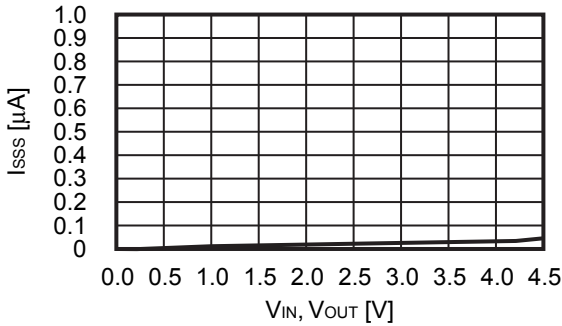
(3) Current consumption during power-off ( I_{SS3} ) vs. Operating input voltage ( V_{IN} ), Output voltage ( V_{OUT} )
