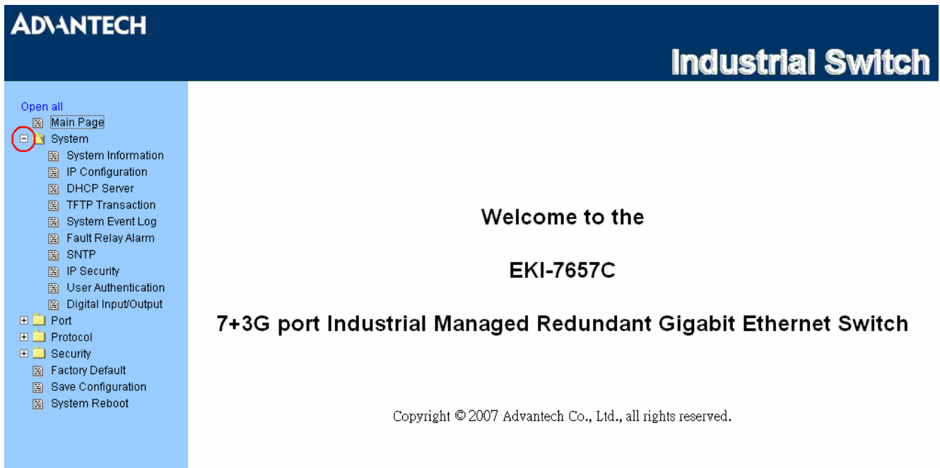
Figure 3.3-3 Main page
