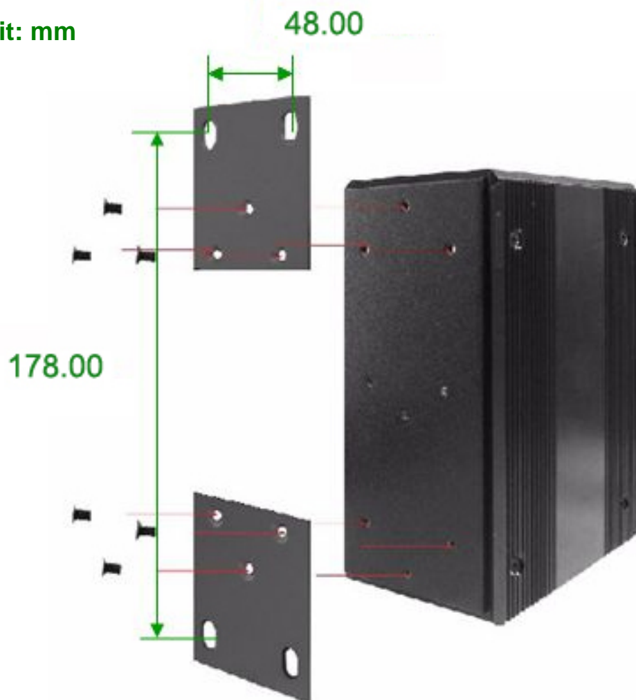
Figure 2.5: Combine the Metal Mounting Kit
