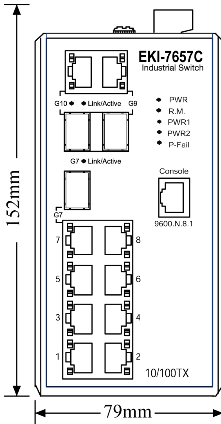
Figure 2.1: Front View
