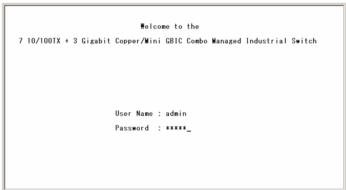
Figure 3.1-4 Login Screen: RS-232 Configuration
