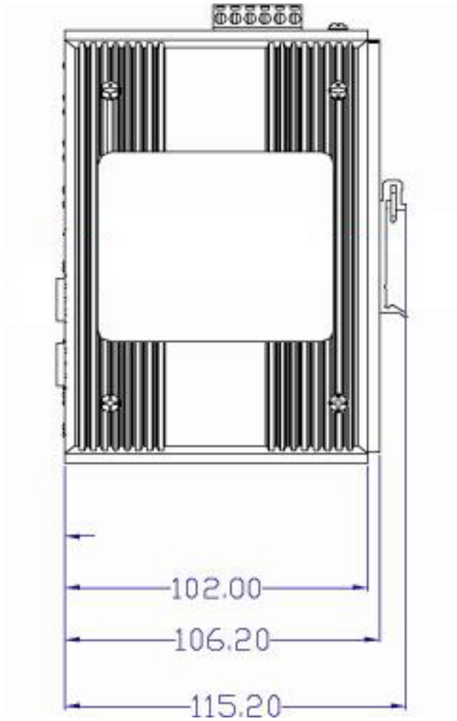
Figure 2.2: Side View
