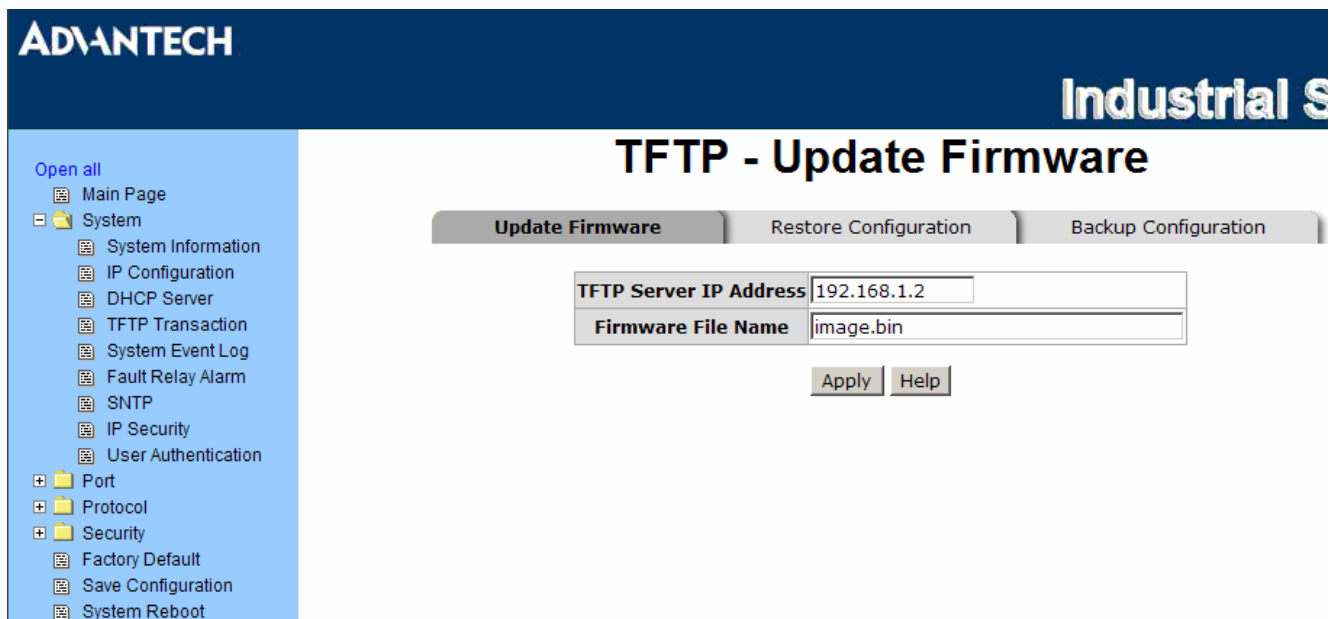
Figure 3.3-9 TFTP – Update Firmware
