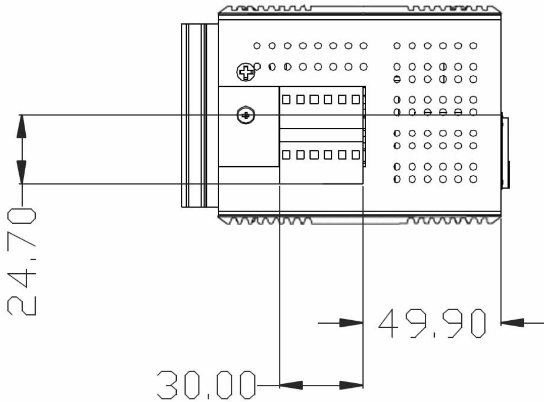
Figure 2.4: Top View
