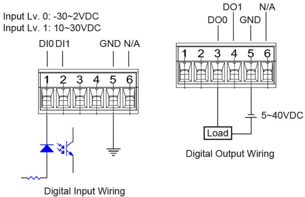
Figure 2.14: Pinouts of the DIDO Connector
