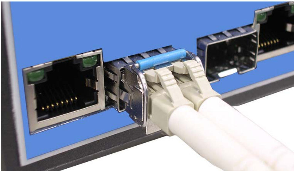
Figure 2.10: LC connector to the transceiver
