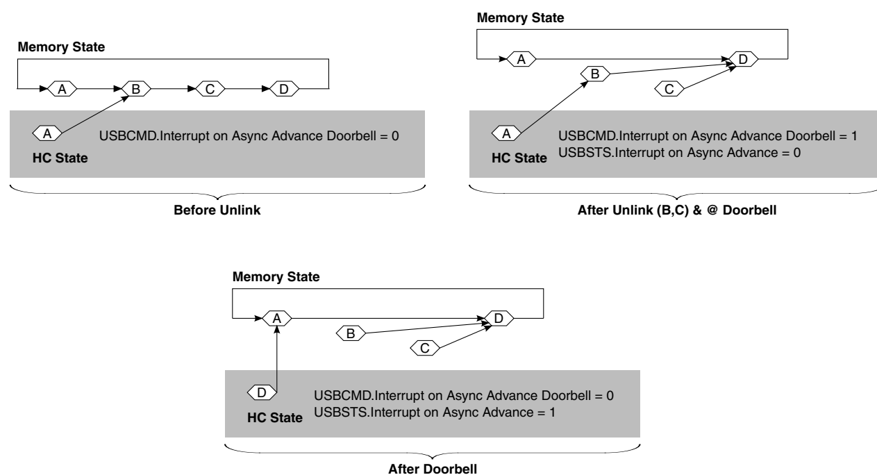
Figure 11-73. Generic Queue Head Unlink Scenario
