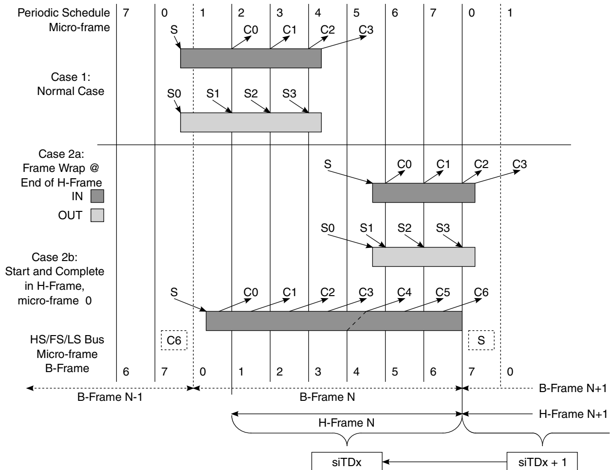
Figure 11-84. Split Transaction, Isochronous Scheduling Boundary Conditions
