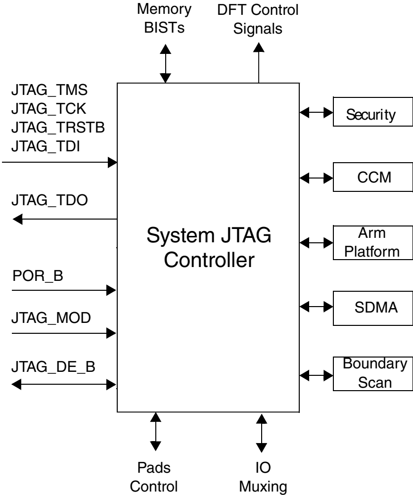
Figure 4-26. SJC Connections
