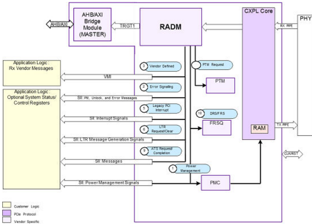
Figure 3-30 Message Reception: RC Mode
