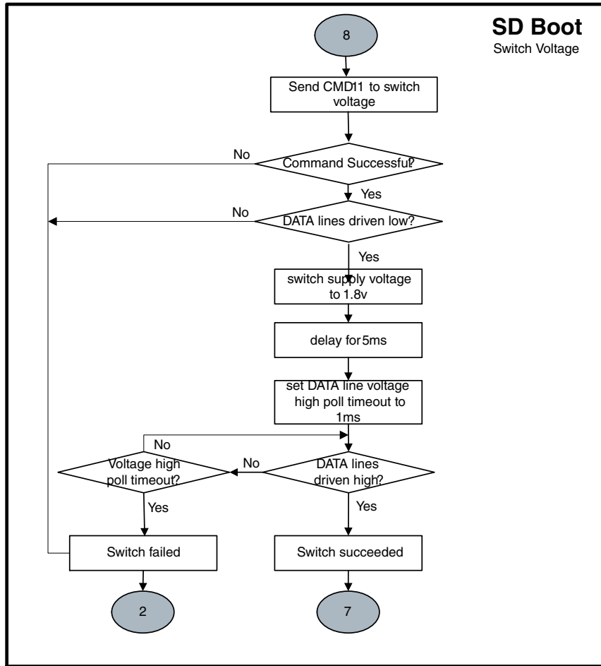
Figure 6-33. Expansion device (SD/eSD/SDXC) boot flow (3 of 6) part 2
