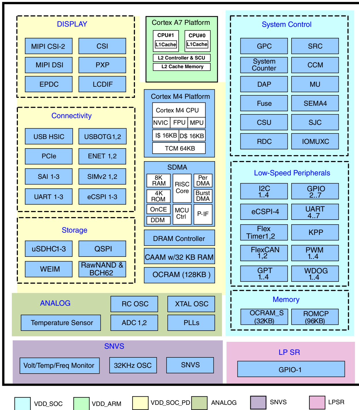
Figure 5-10. Power Domains
