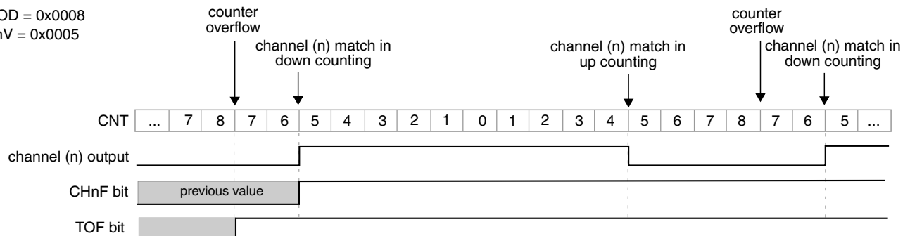
Figure 12-28. CPWM signal with ELSnB:ELSnA = 1:0
