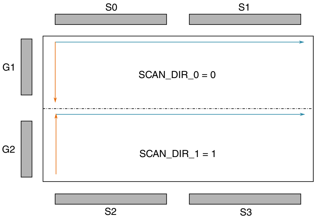
Figure 13-79. Dual-Scan Method (Scan = 01)
