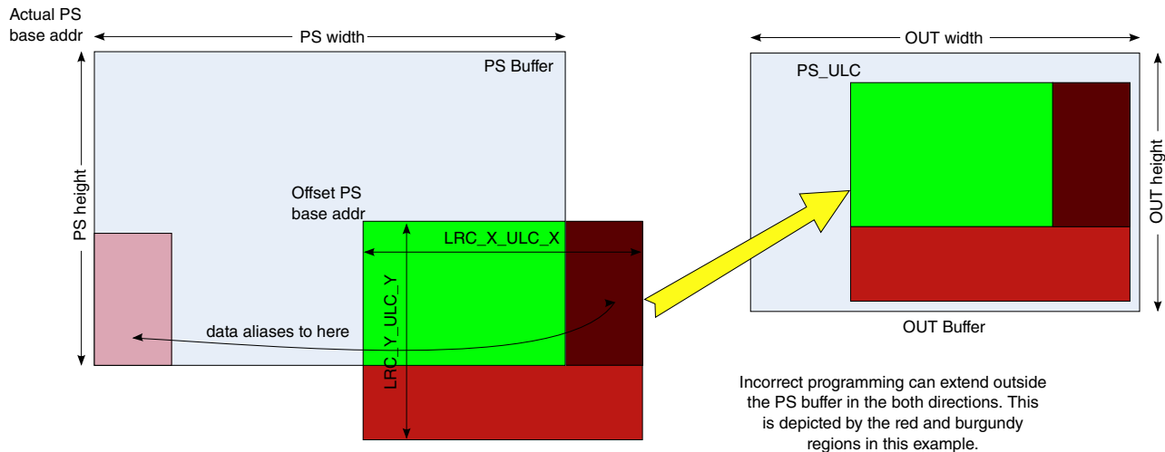
Figure 13-106. Example with Invalid Parameters
