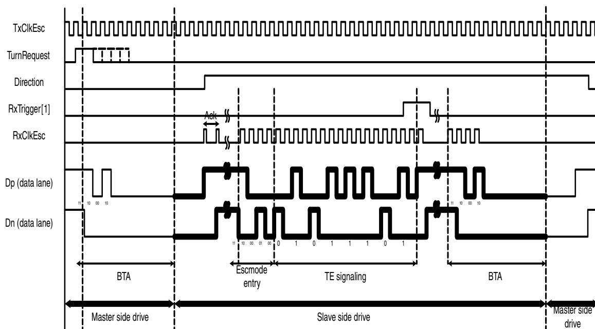
Figure 13-45. TE Signaling
