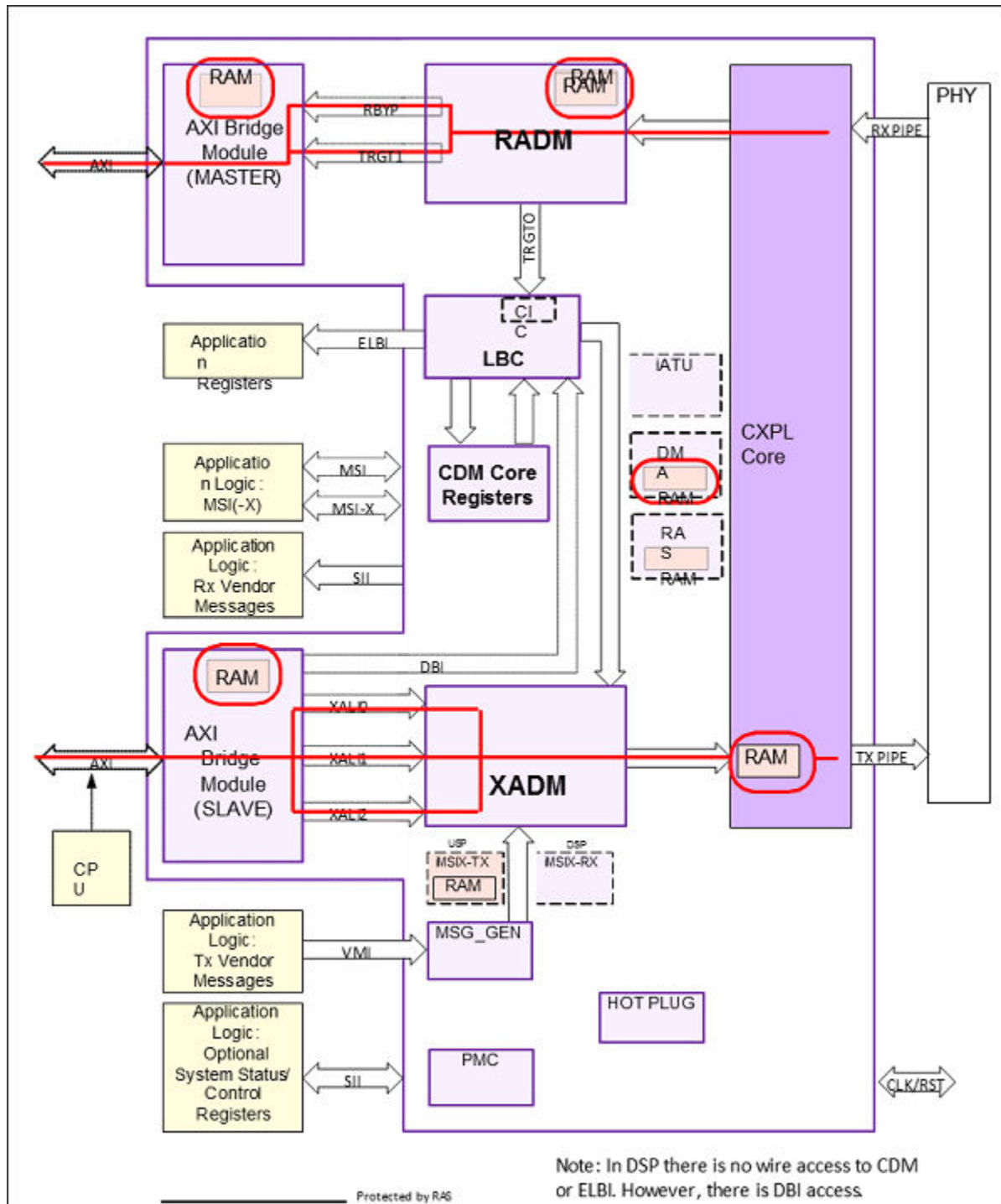
Figure 3-18 RAS DP Protection Coverage
