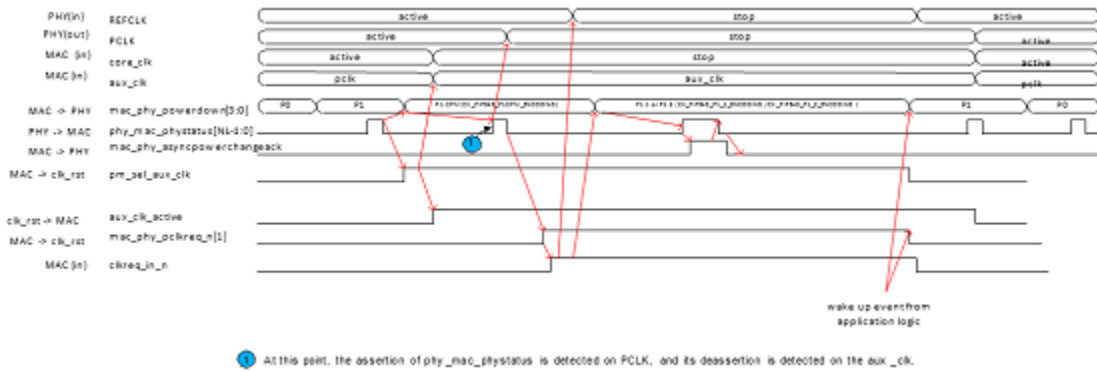
Figure 3-47 PIPE 4.3 L1 SS Operation (CX_PIPE43_ASYNC_HS_BYPASS=0 / CX_PIPE43_P0_P1CPM=1)
