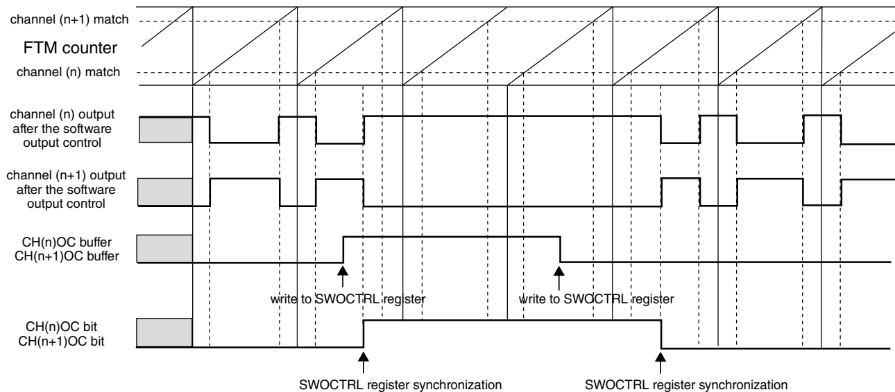
Figure 12-70. Example of software output control in Combine and Complementary mode
