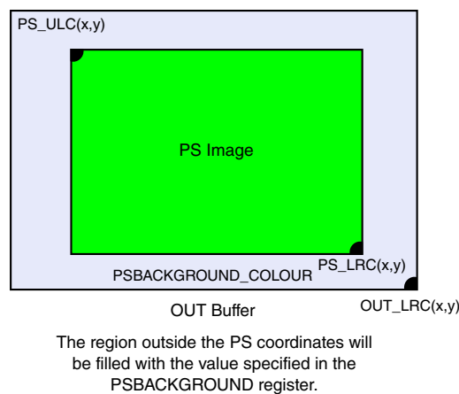
Figure 13-104. OUT Buffer
