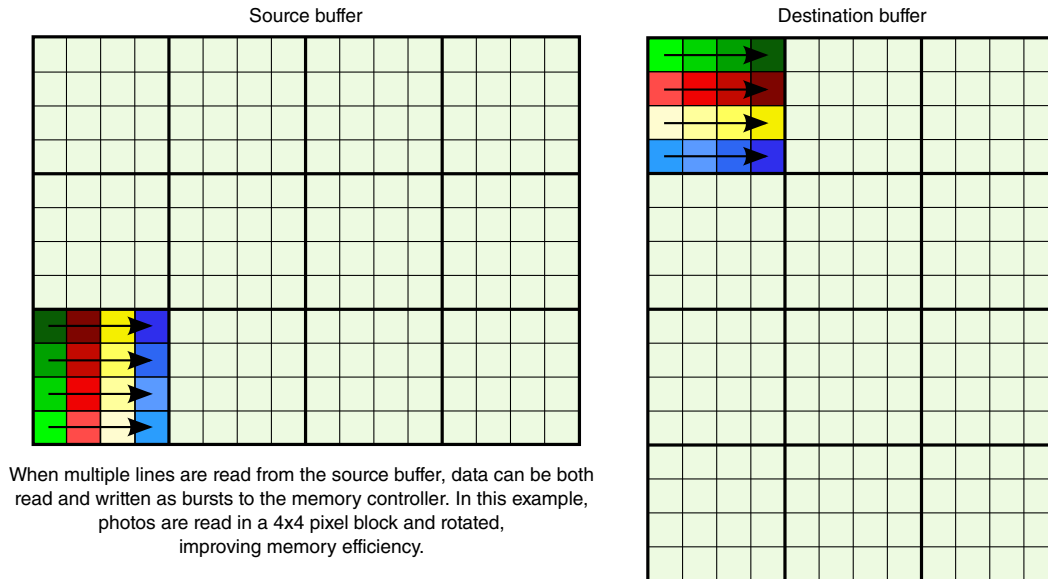
Figure 13-96. Rotated Sub-blocks
