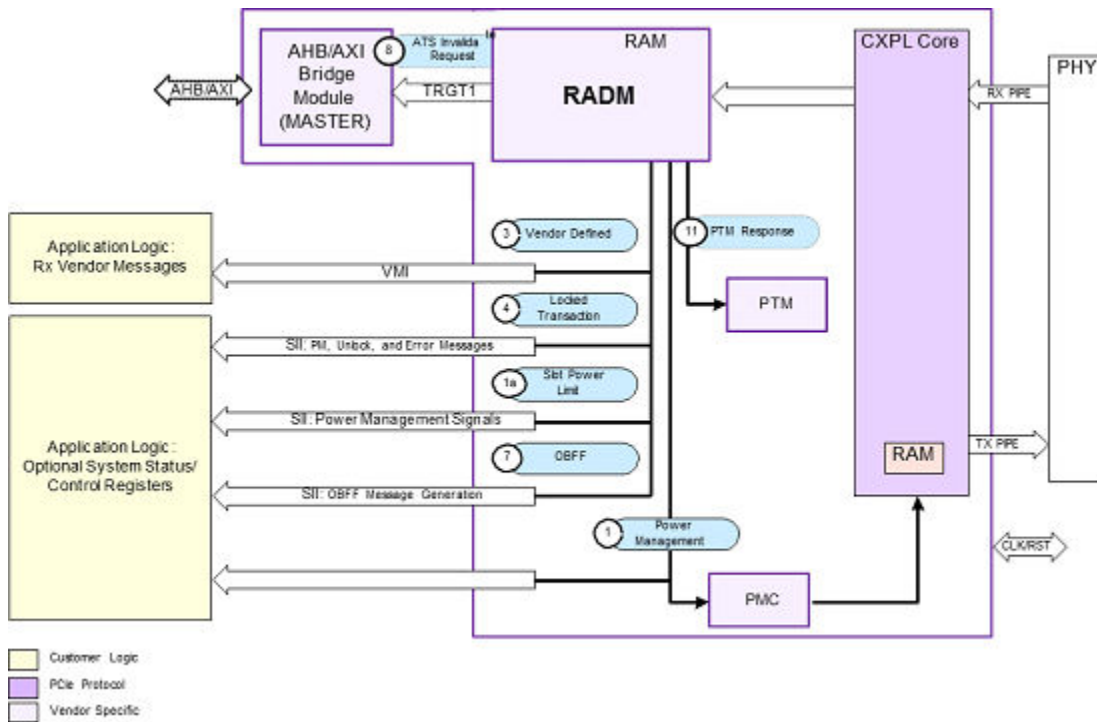
Figure 3-30 Message Reception: RC Mode
