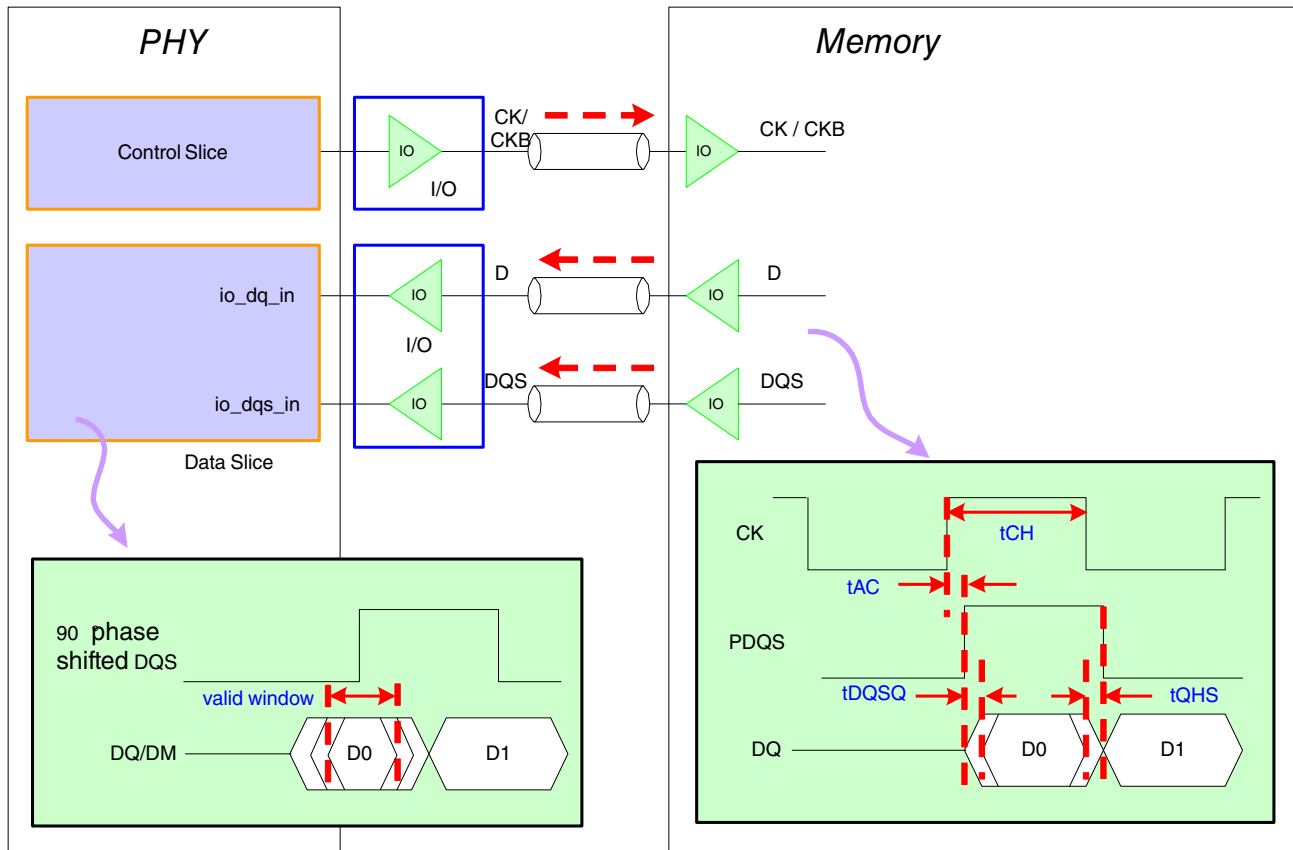
Figure 9-13. Block Diagram of the Read Path
