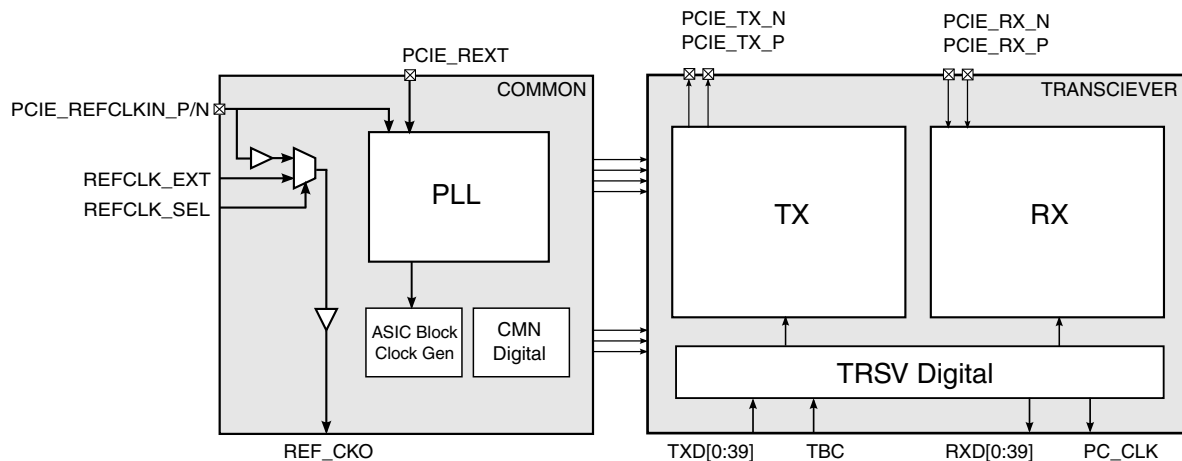
Figure 11-53. Block Diagram
