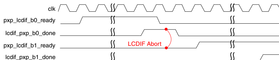
Figure 13-102. LCDIF Abort
