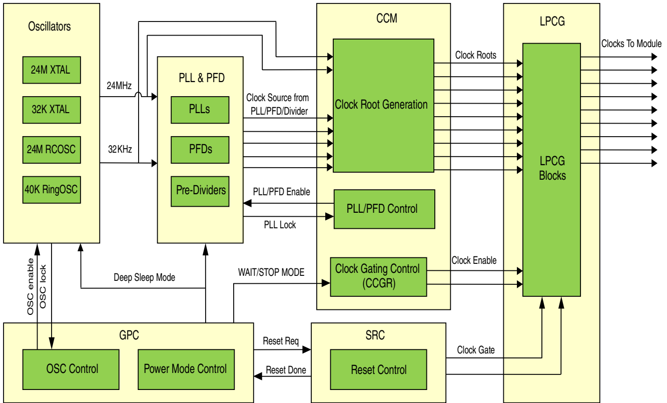
Figure 5-1. Clock System
