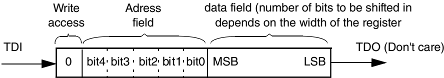
Figure 4-29. TDI/TDO on write access
