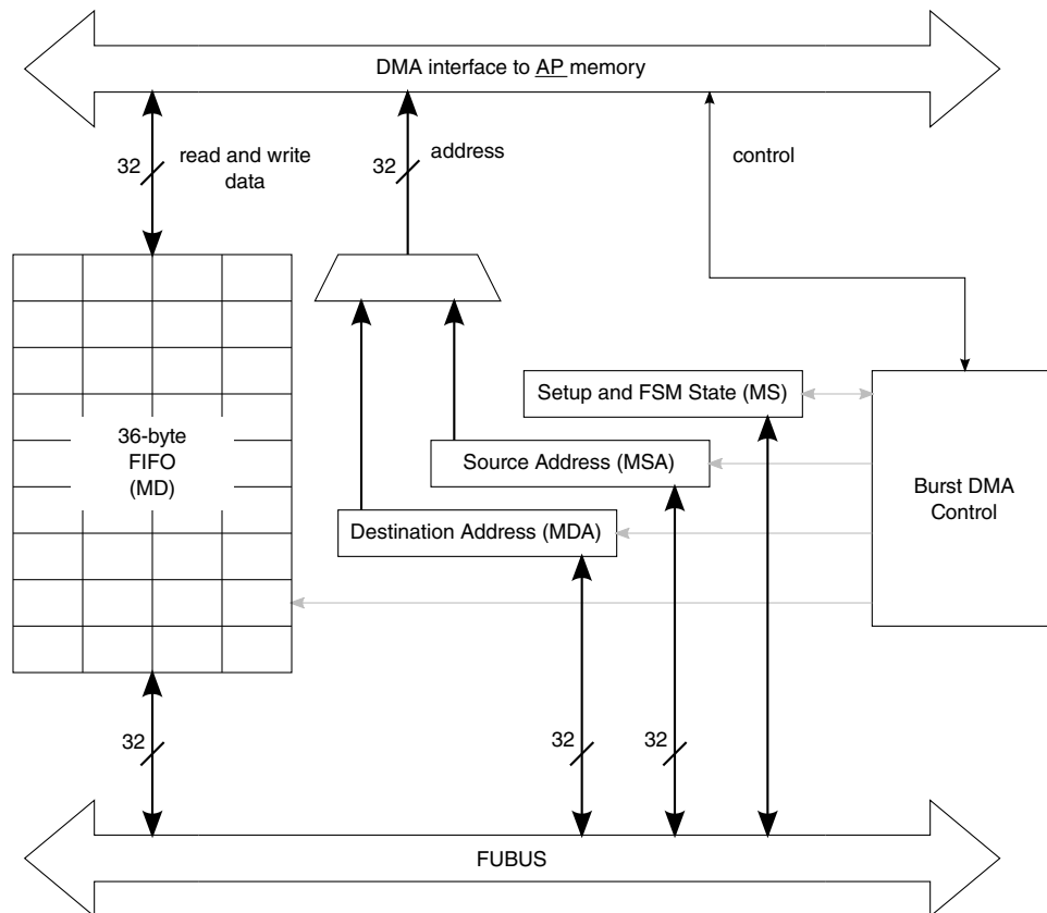
Figure 7-8. Burst DMA Structure
