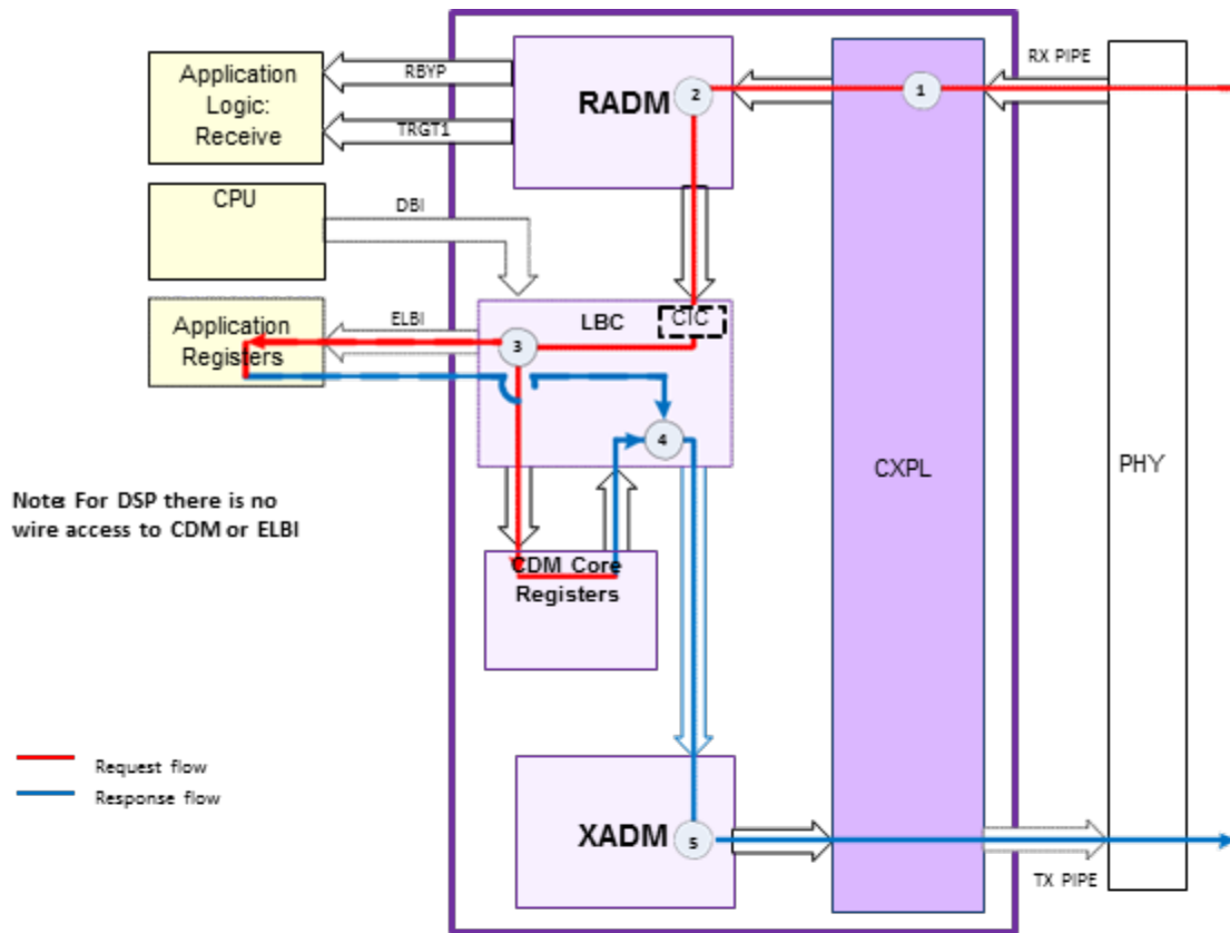
PCIe Wire Access to CDM Registers or ELB(USP)
