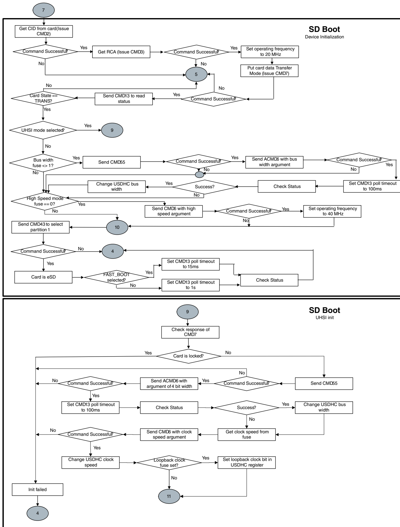
Figure 6-34. Expansion device (MMCSD/eSD/SDXC) boot flow (4 of 6) i.MX 7Dual Applications Processor Reference Manual, Rev. 1, 01/2018
