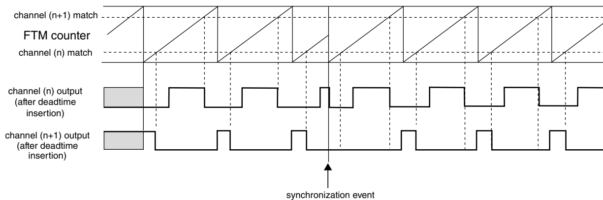
Figure 12-63. FTM counter synchronization
