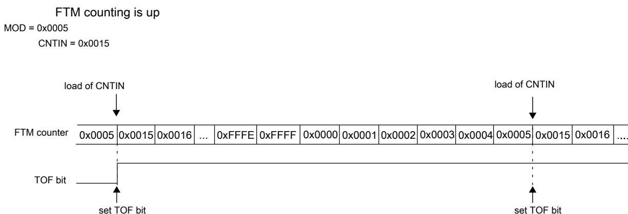
Figure 12-11. Example of up counting when the value of CNTIN is greater than the value of MOD
