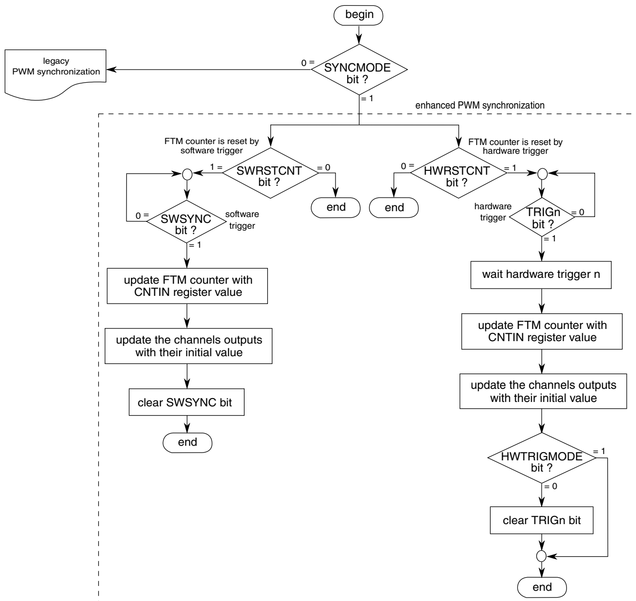
Figure 12-64. FTM counter synchronization flowchart
