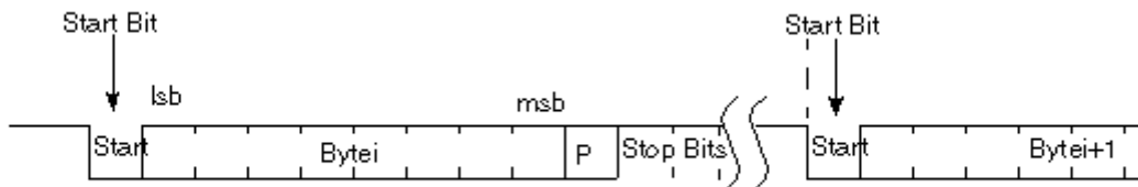
Figure 11-44. Start Bit Diagram
