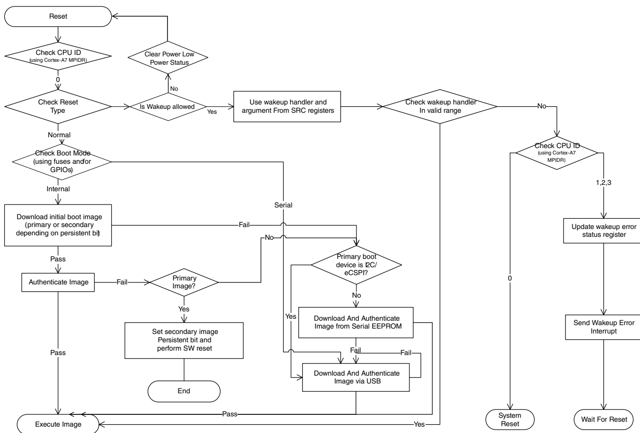
Figure 6-19. Boot flow
