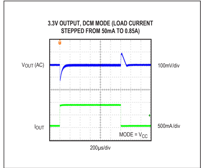
Figure 9. MAX17505 3.3V Output, 50mA to 0.85A Load Transient (DCM Mode)
