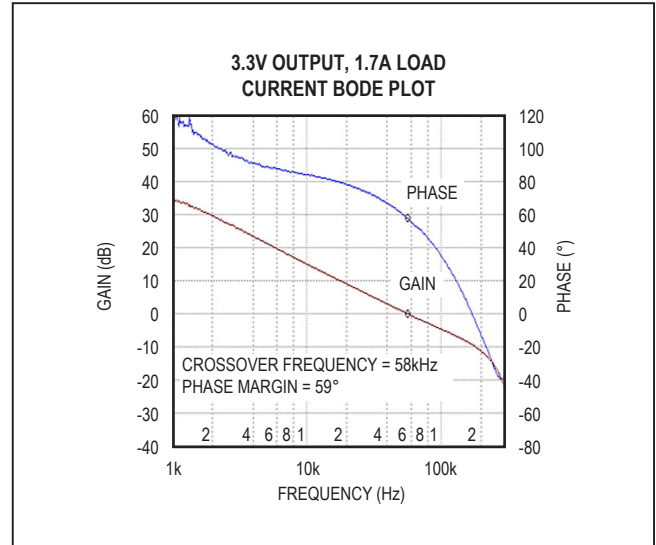
Figure 6. MAX17505 3.3V Output Full Load Bode Plot ( V_{IN} = 24V )
