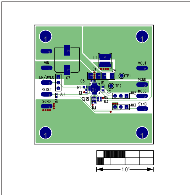
Figure 13. MAX17505 3.3V Output EV Kit Component Side PCB layout
