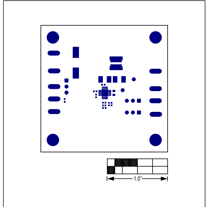
Figure 17. MAX17505 3.3V Output EV Kit Component Placement Guide—Top Solder Mask
