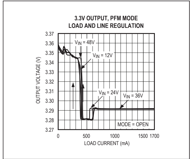
Figure 3. MAX17505 3.3V Output Load and Line Regulation (PFM Mode)
