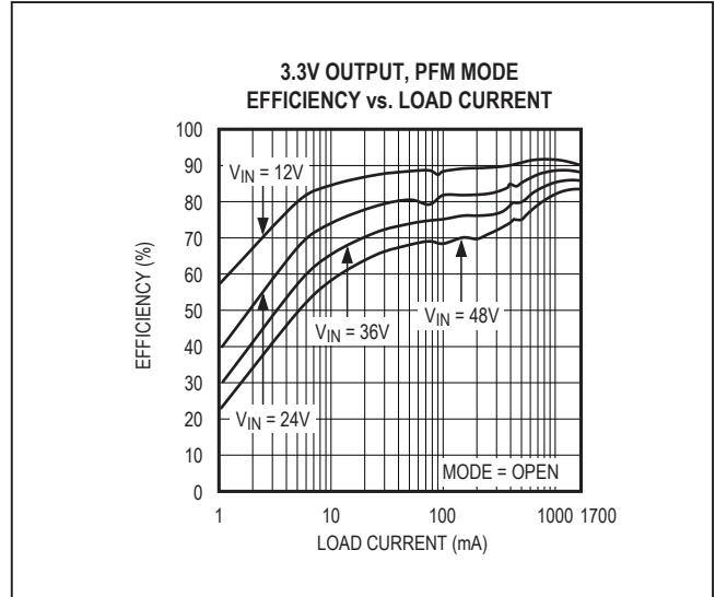
Figure 4. MAX17505 3.3V Output Efficiency (PFM Mode)
