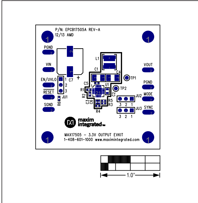
Figure 12. MAX17505 3.3V Output EV Kit Component Placement Guide—Component Side
