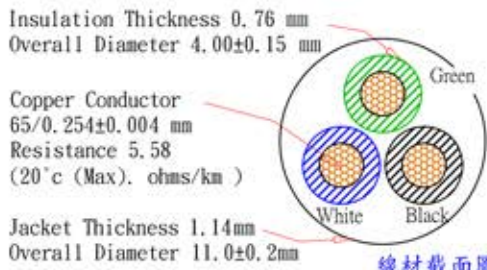
線材截面圖 (Wire Cross-Section)
