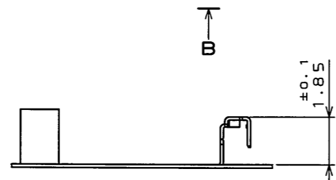
VIEW B (SCALE 2:1)
