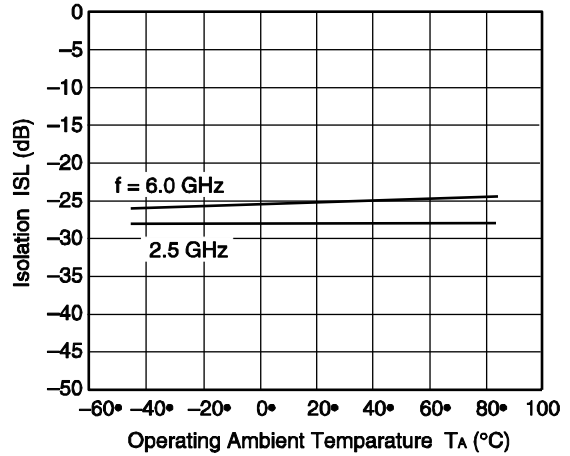
RFC-RF1/RF2 ISOLATION vs. OPERATING AMBIENT TEMPERATURE
