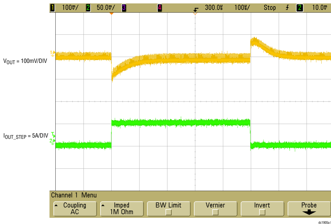
Figure 5. Measured Channel 1 Load Transient V_{IN} = 12\text{V} , V_{OUT1} = 1.0\text{V} , I_{STEP} = 0\text{A to } 5\text{A} , di/dt = 5\text{A}/\mu\text{s}
