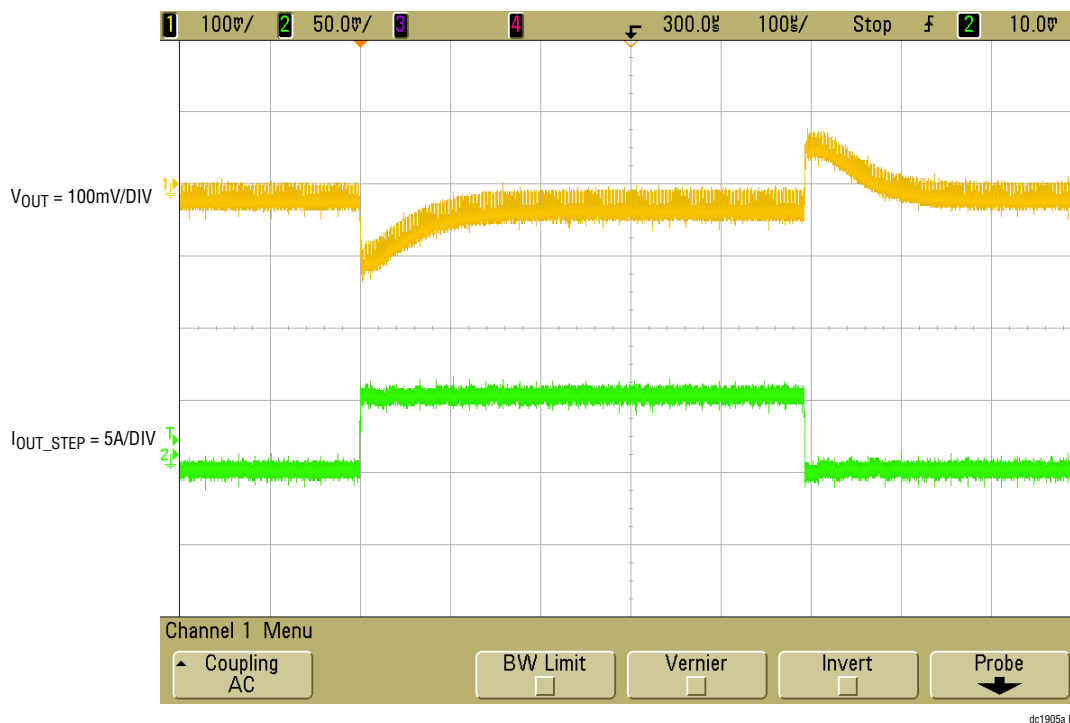
Figure 6. Measured Channel 2 Load Transient V_{IN} = 12\text{V} , V_{OUT1} = 1.2\text{V} , I_{STEP} = 0\text{A to } 5\text{A} , di/dt = 5\text{A}/\mu\text{s}
