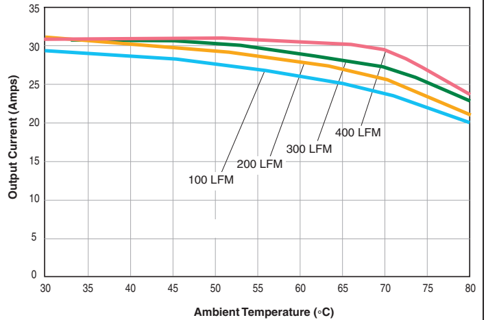
UCQ-1.5/25-D48 Maximum Current Temperature Derating
