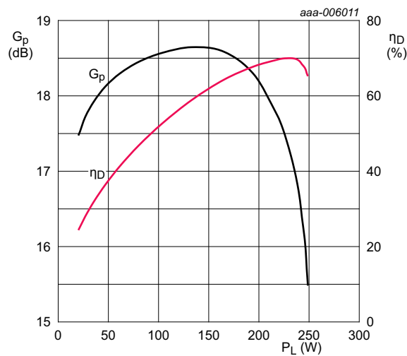
V_{DS} = 32 \text{ V}; I_{Dq} = 100 \text{ mA}; f = 1300 \text{ MHz}; t_p = 100 \mu\text{s}; \delta = 20\%.
