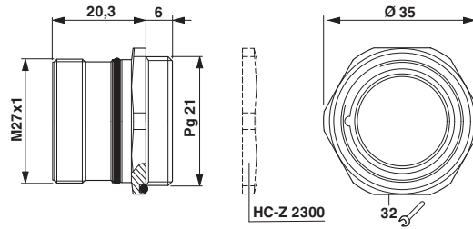
Dimensioned drawing
