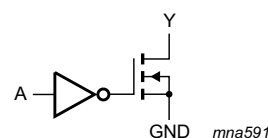
Fig 3. Logic diagram
