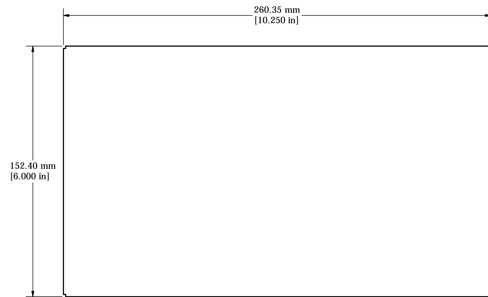
TOP VIEW OF ASSEMBLY
