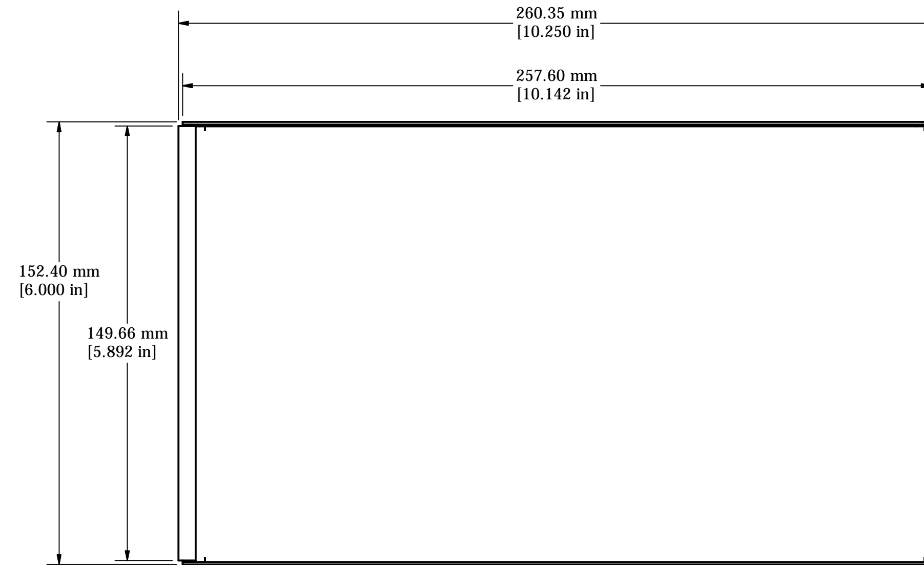
BOTTOM VIEW OF ASSEMBLY
