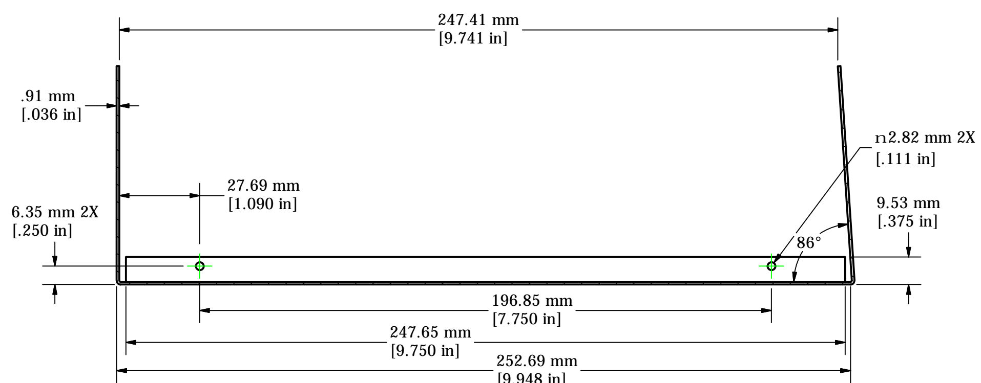
SECTION A-A SIDE SECTION VIEW OF EXPLODED ASSEMBLY
