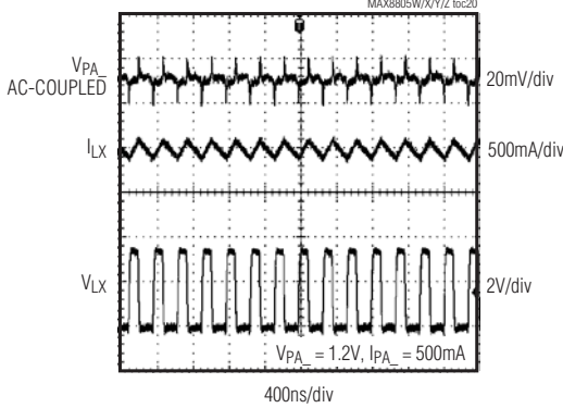
PA STEP-DOWN CONVERTER HEAVY-LOAD SWITCHING WAVEFORMS (MAX8805X/MAX8805Z)
