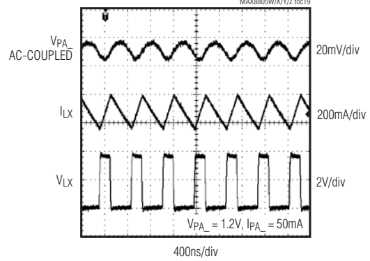
PA STEP-DOWN CONVERTER LIGHT-LOAD SWITCHING WAVEFORMS (MAX8805W/MAX8805Y)
