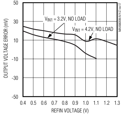
REFIN vs. REFIN TO OUT GAIN (MAX8805W)
