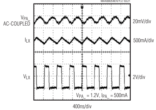
PA STEP-DOWN CONVERTER HEAVY-LOAD SWITCHING WAVEFORMS (MAX8805W/MAX8805Y)
