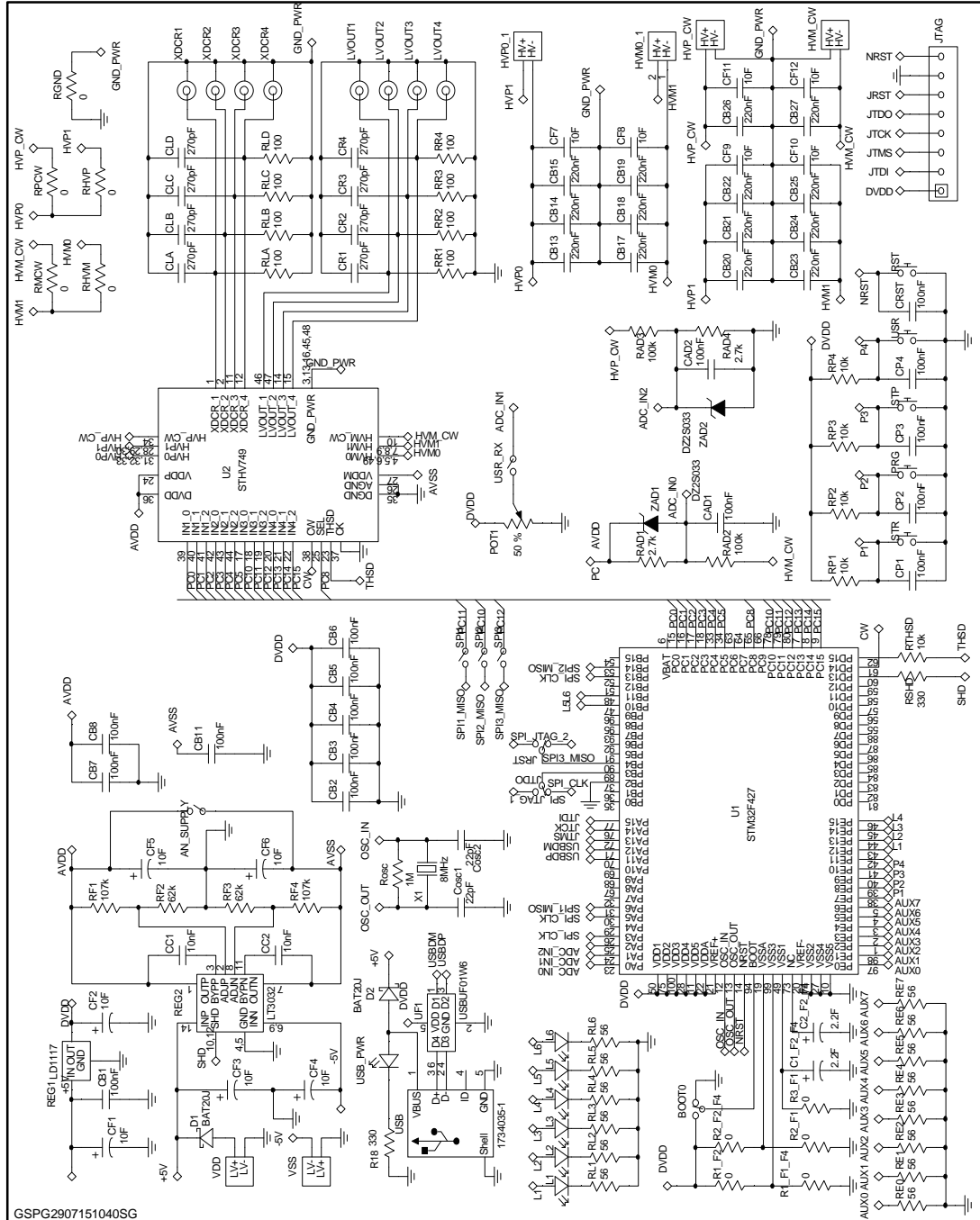
Figure 1: STEVAL-IME012V1 circuit schematic
