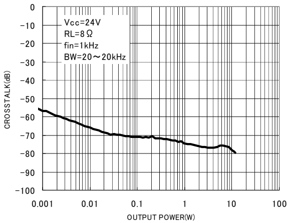
Fig.5 Output power—Crosstalk
