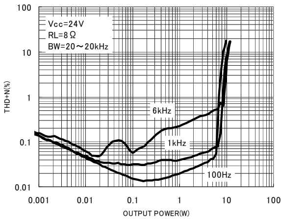
Fig.3 Output power—THD+N
