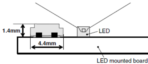
Explanatory diagram of the connector mounted on a circuit board
