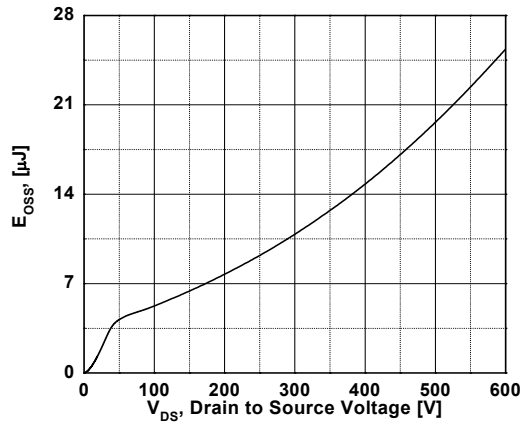
Figure 16. E_{oss} vs. Drain to Source Voltage
